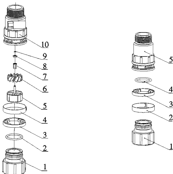
5447007 Flow Meter
