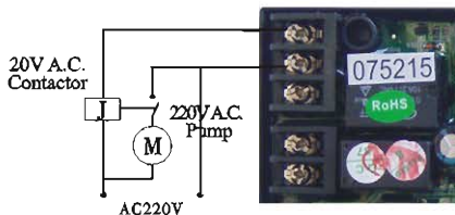
Figure3-8 Wiring diagram of inlet pressure pump (<5A)
